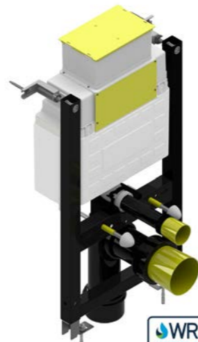
Keytec 0.82m WC Frame With front access dual flush cistern.
