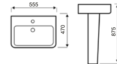
Basin & Pedestal
