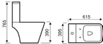
Close-Coupled WC
