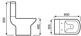
Close-Coupled WC
