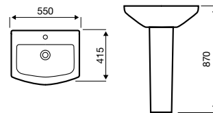
Basin & Pedestal
