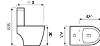
Close-Coupled WC
