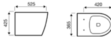
Wall Hung WC
