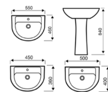
Semi-Recessed Basin
