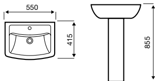
Basin & Pedestal
