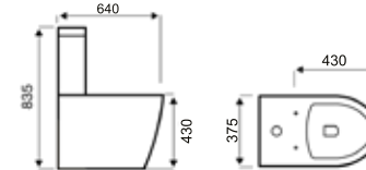
Close-to-Wall WC
