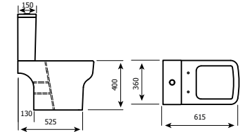
Back-to-Wall WC
