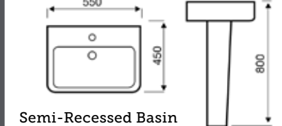
Basin & Pedestal
