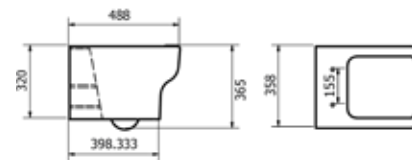
Wall-Hung WC
