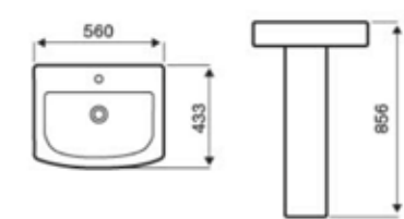
Basin & Pedestal
