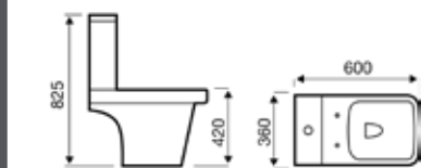
Close-to-Wall WC
