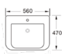
Semi-Recessed Basin
