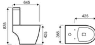
Close-to-Wall WC
