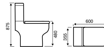
Back-to-Wall WC
