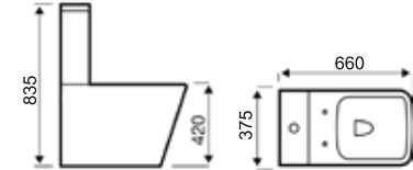
Back-to-Wall WC
