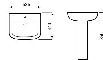
Basin & Pedestal
