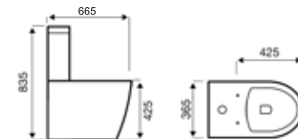
Back-to-Wall WC
