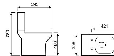
Back-to-Wall WC
