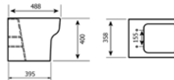
Wall-Hung WC
